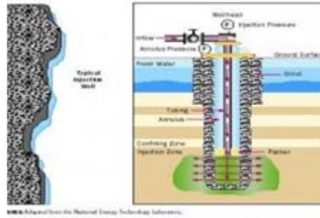
DIAGRAM OF INJECTION WELL
